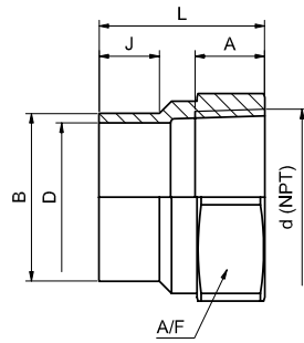
Dimensions Table Female Adaptor
