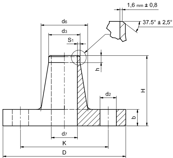
Weld preparation applicable to S_1 \geq 3,0 \text{ mm}
