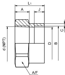
Dimensions Table Female
