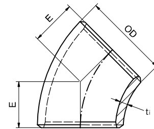
ti = intrados thickness (min) in accordance with EEMUA Publication No. 146: Section 1, Table 1.5
