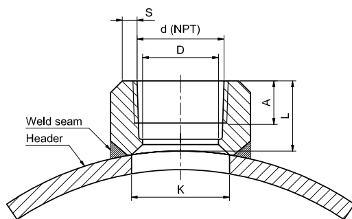
Dimensions Table Threadolets 16/1/2" - 965/38" x 16/1/2" - 57/2" - 16/20 bar
